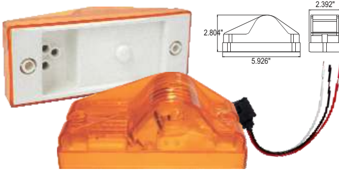
Conector. 7794
